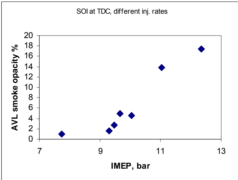
Smoke vs IMEP, SOI at TDC
