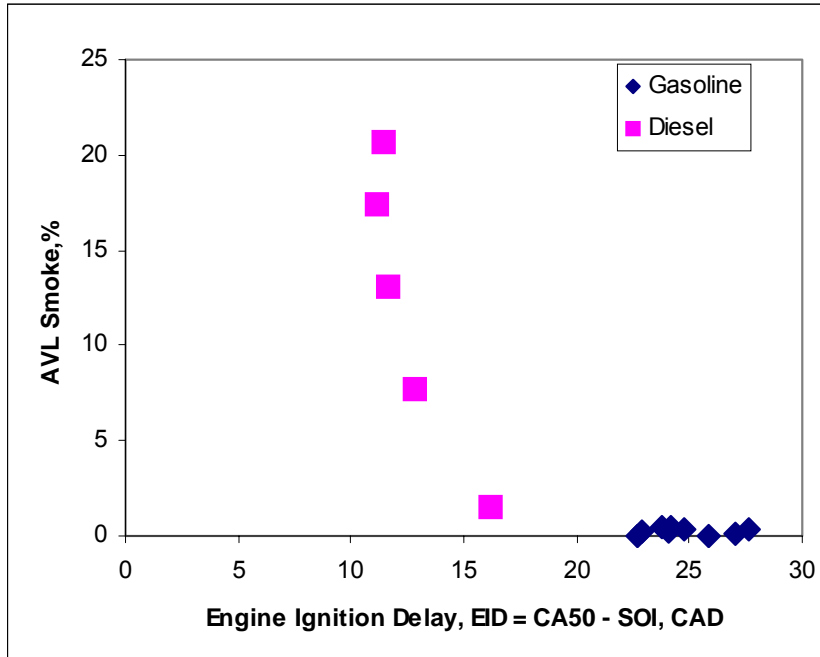
Smoke vs ignition delay
