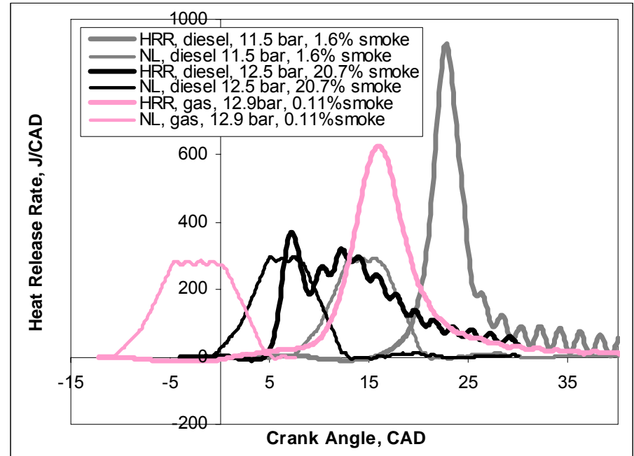
HRR and needle lift for three cases
