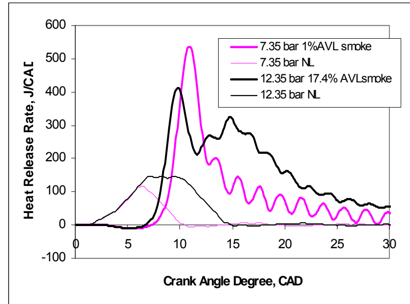
Heat release rate and needle lift for low and high smoke cases
